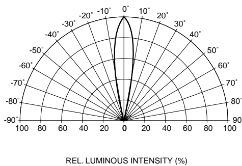
Fig. 5 Radiation Diagram
